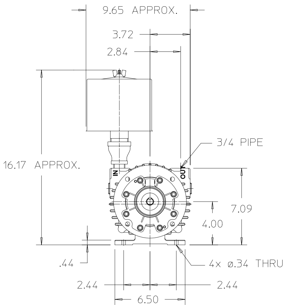
VIEW SHOWN LESS MOTOR
