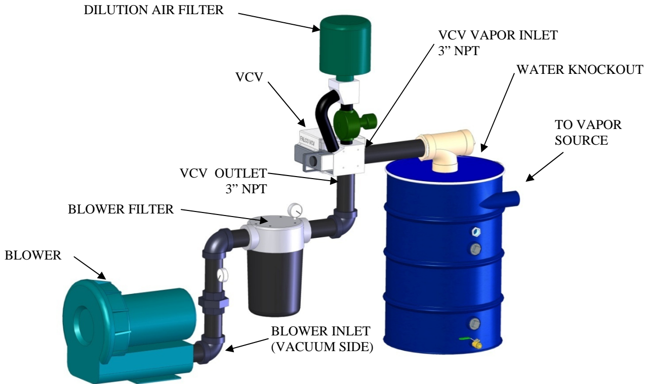
Figure 2 - ALTERNATIVE (LESS DESIRABLE) INSTALLATION
