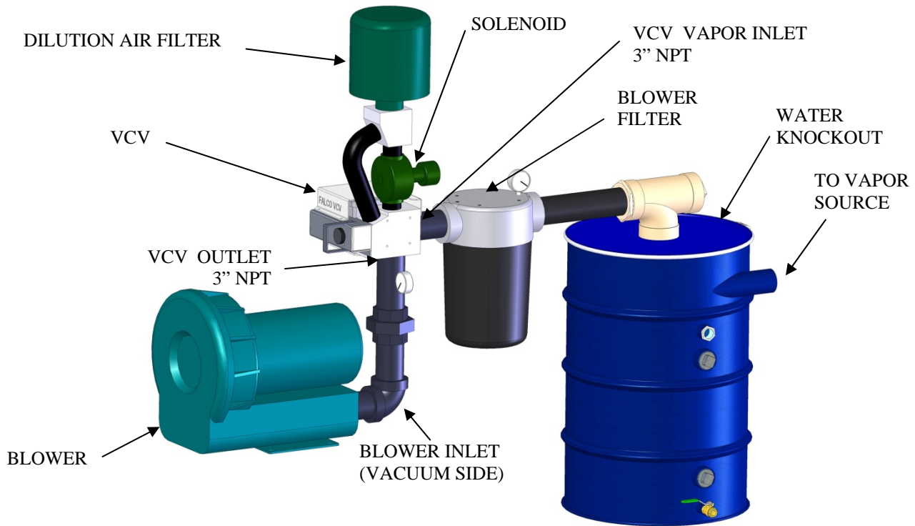
Figure 1 - PREFERRED INSTALLATION
