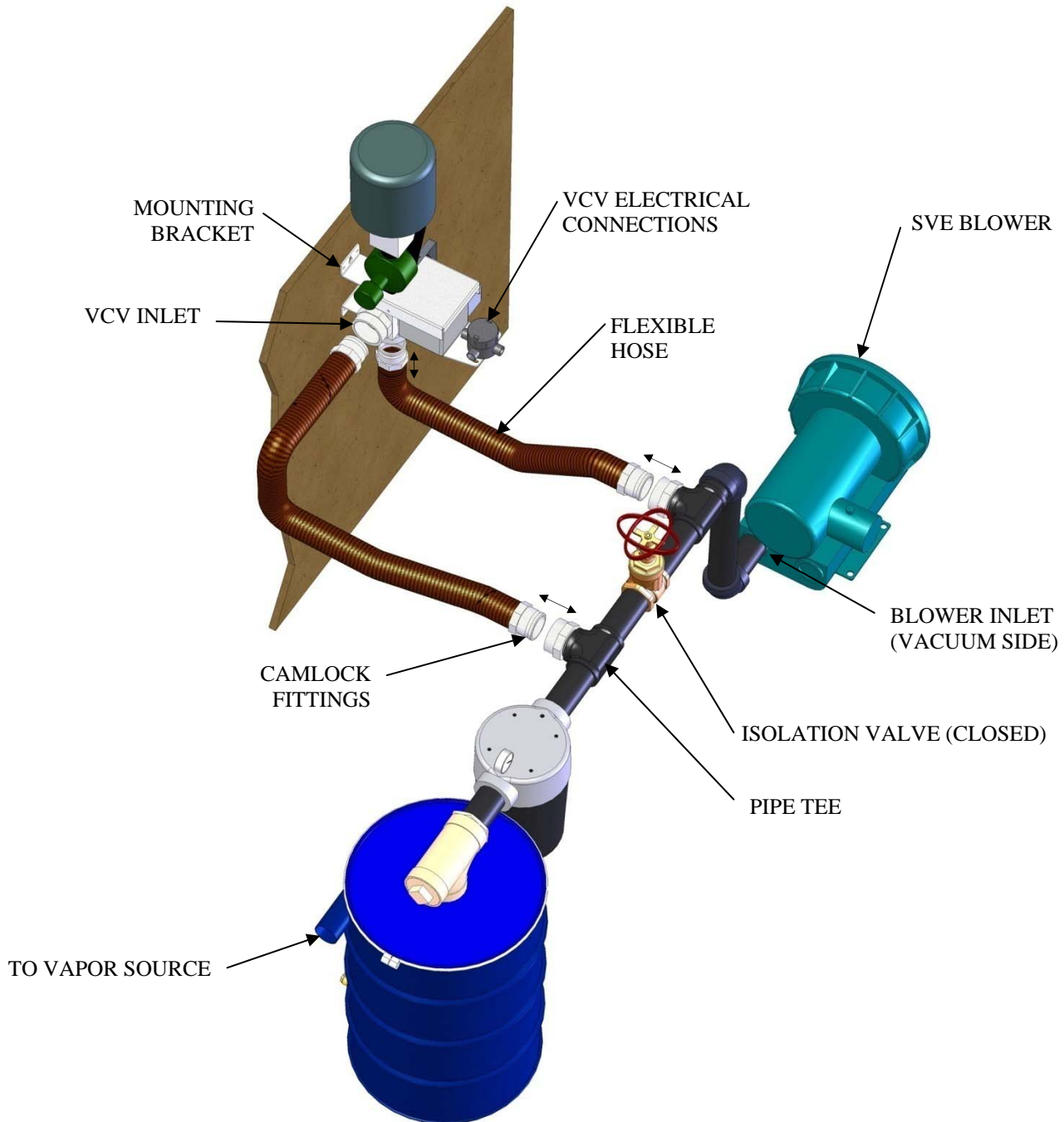
Figure 3 – TEMPORARY INSTALLATION
