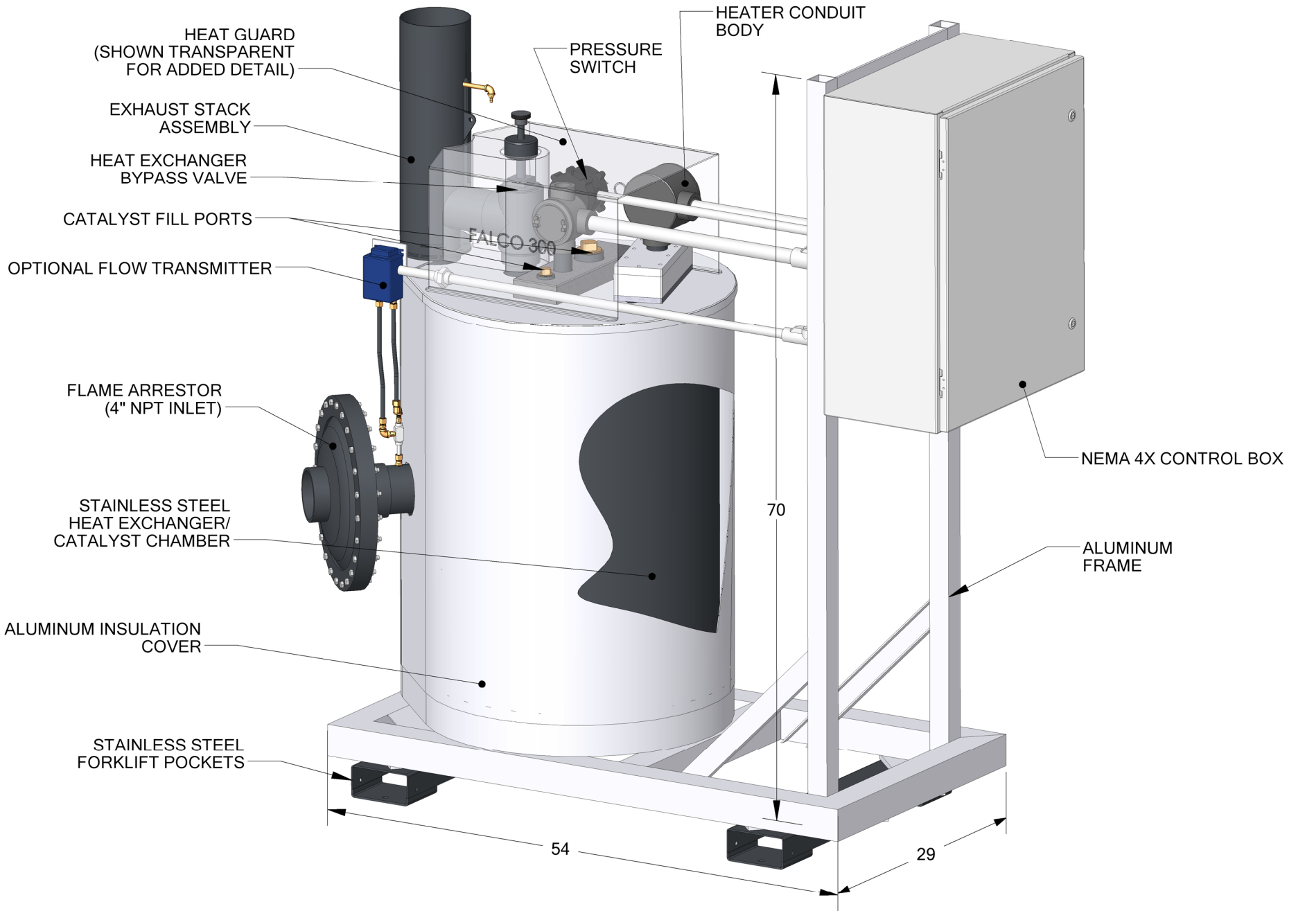
FALCO 300 - MAJOR COMPONENTS
