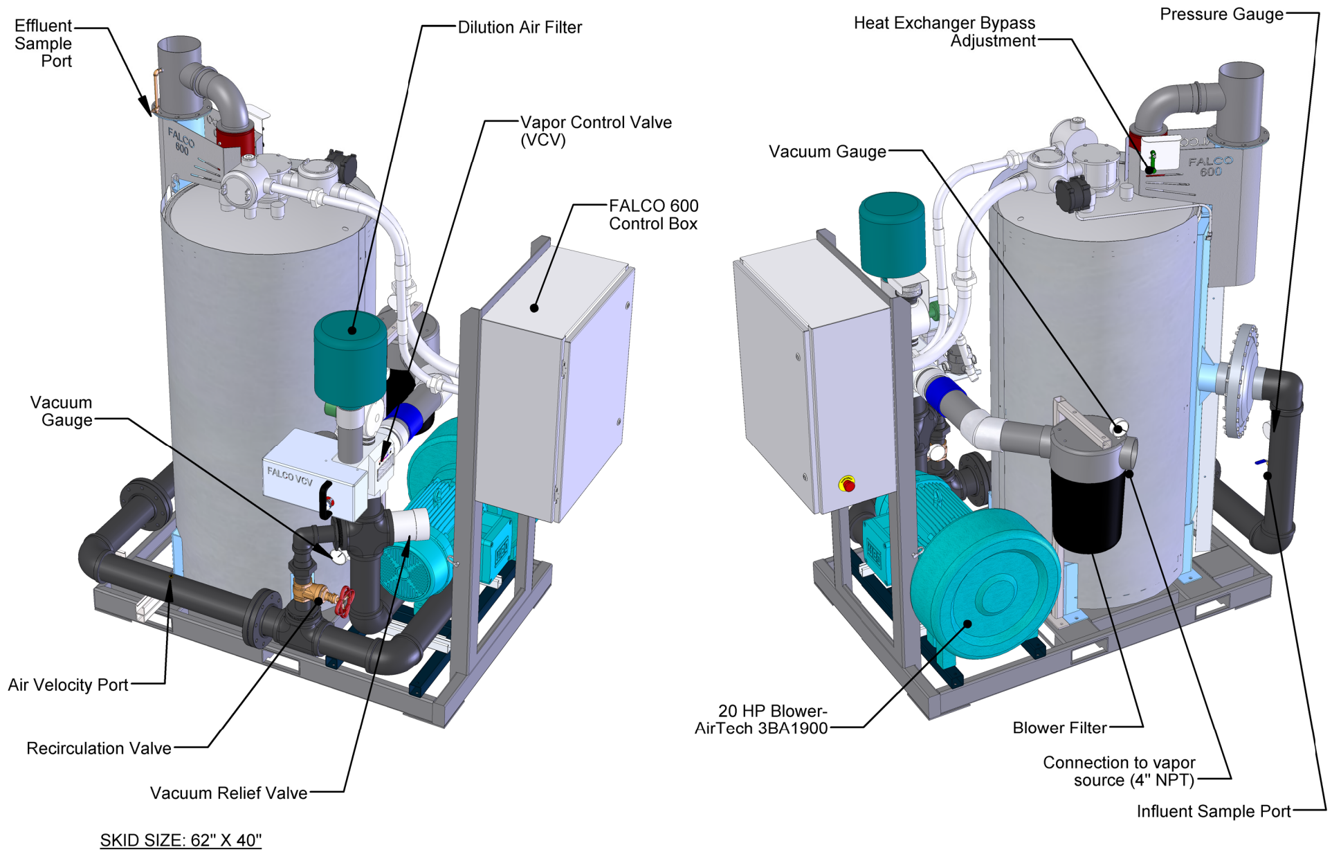
FALCO 600 with Regenerative Blower Assembly
