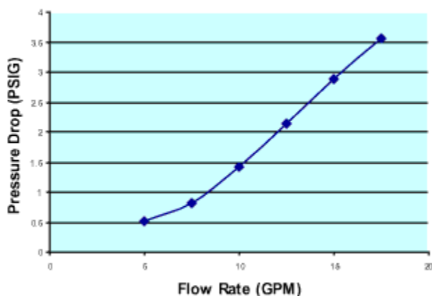
PRESSURE DROP GRAPH (As Filled 8*30 GAC)
