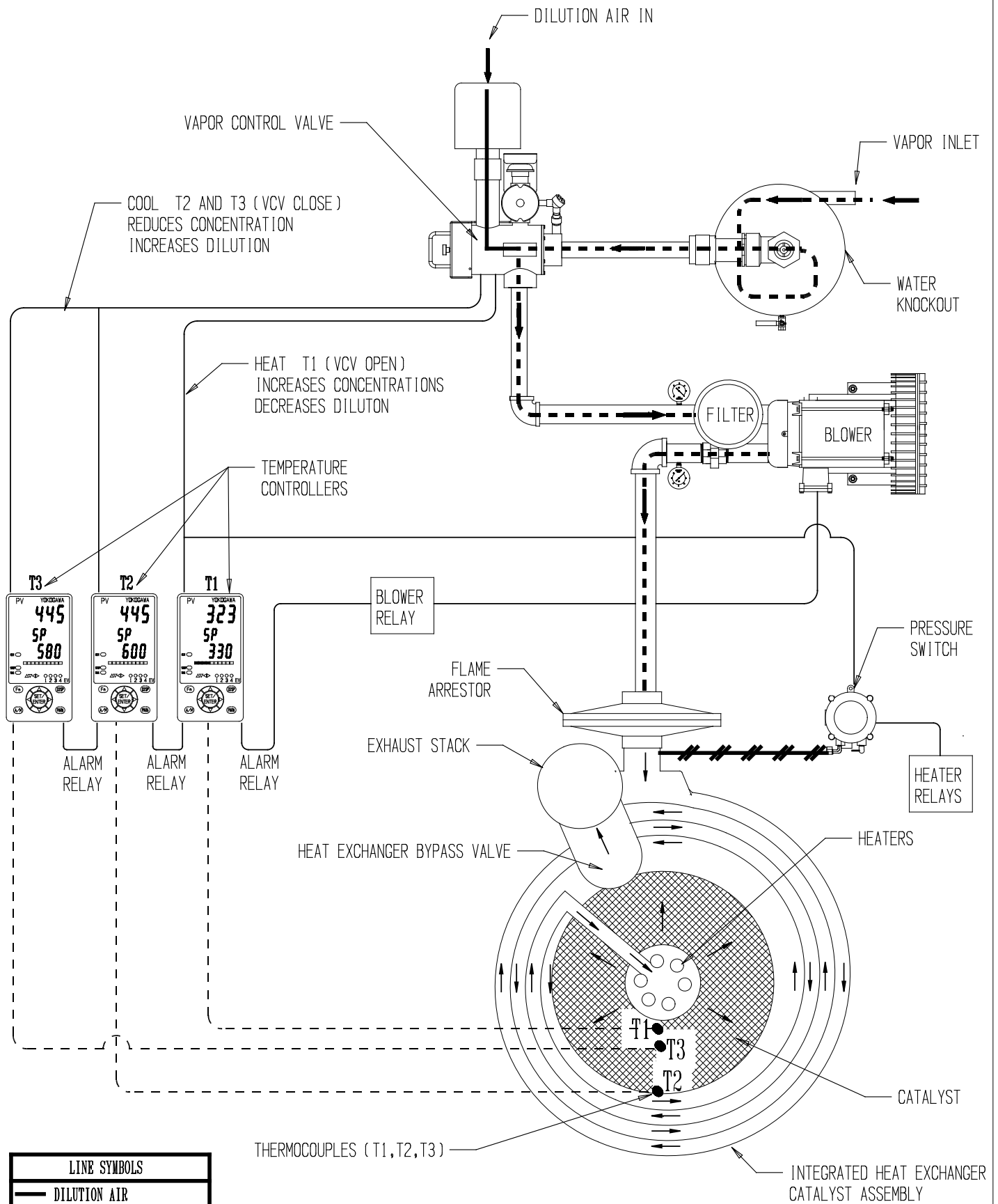
FIGURE 3: FALCO 600 FLOW AND CONTROL
