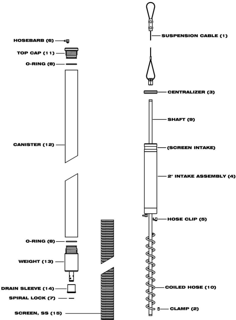
Figure 7-1: Standard 2" PRC Skimmer Assembly
