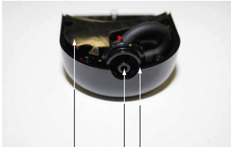
Figure 39 Pump Reassembly
