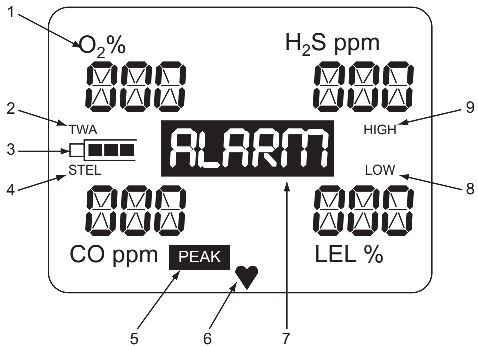
Figure 23 LCD Indicators
