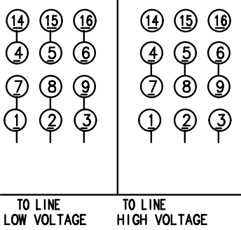
WIRING DIAGRAM
