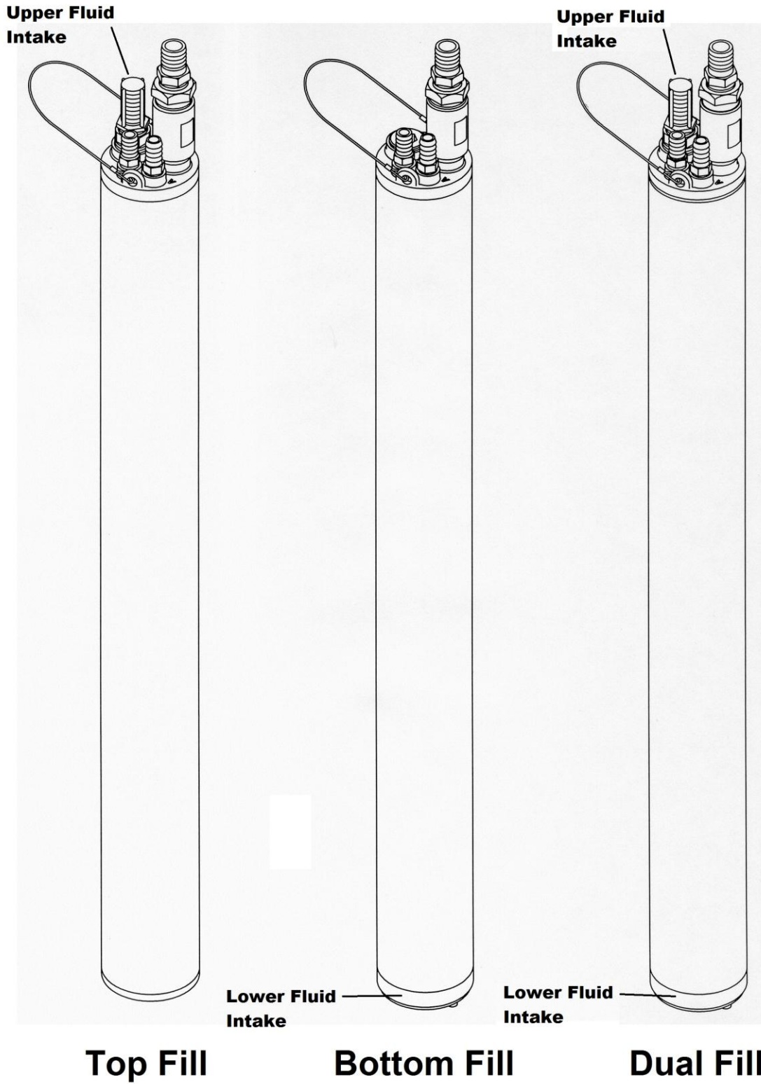
Figure 1-1 3.5 Auto-Reclaimer Models
