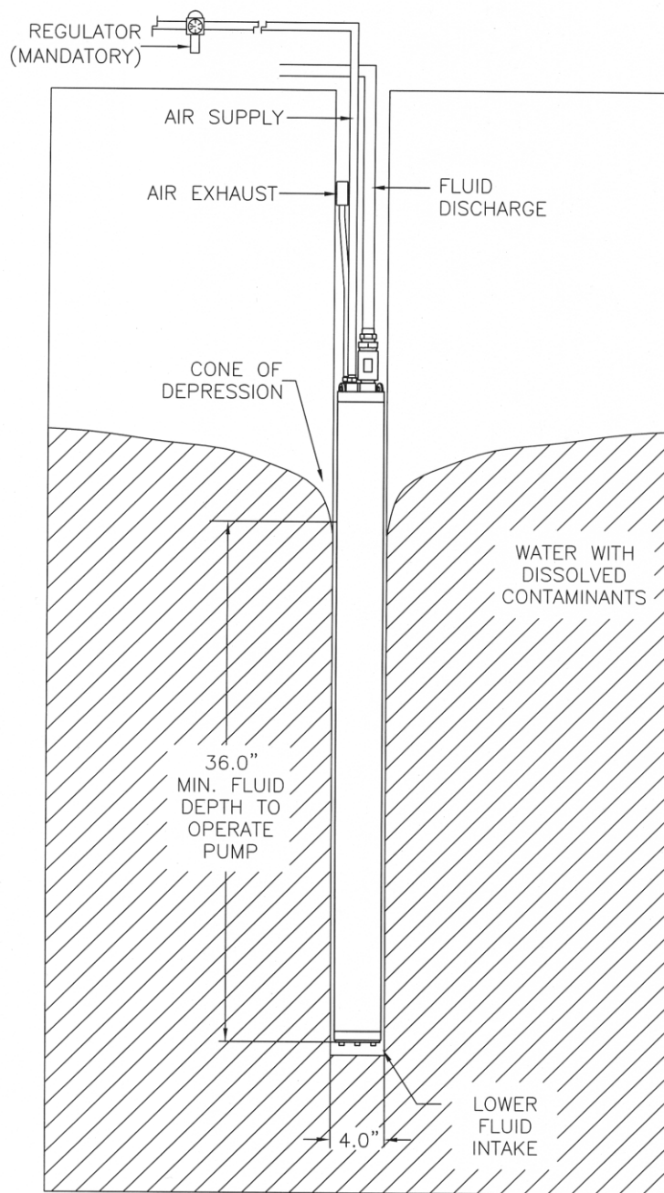
Figure 2-4 48" Bottom Fill Auto-reclaimer in the well
