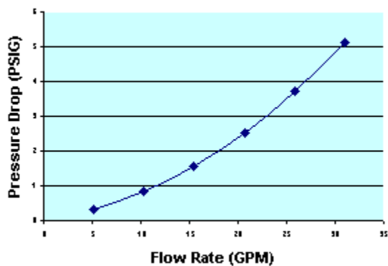
PRESSURE DROP GRAPH (As Filled - 8*30 GAC)
