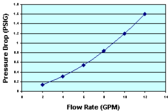
PRESSURE DROP GRAPH (As Filled - 8*30 GAC)
